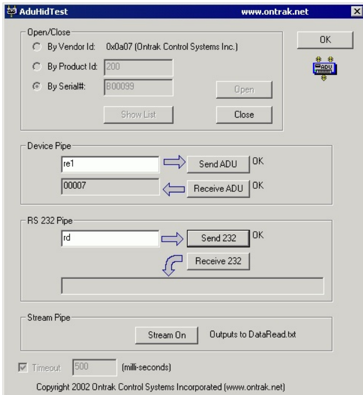
Figure 6: Sending "rd" Command to RS232 Pipe
